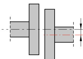
Radial misalignment
